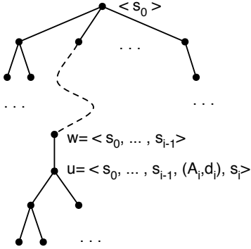
Figure 1: Canonical Tree.
