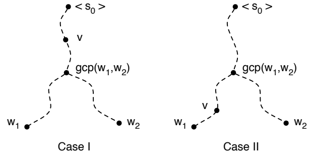
Figure 3: Towards the proof of Lemma 10.
