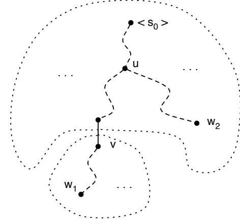
Figure 4: Towards the proof of Claim 1.
