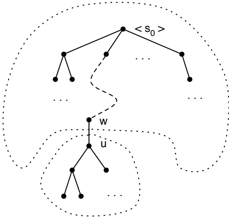
Figure 2: Two equivalence classes of relation \sim_{(u,a)} .
