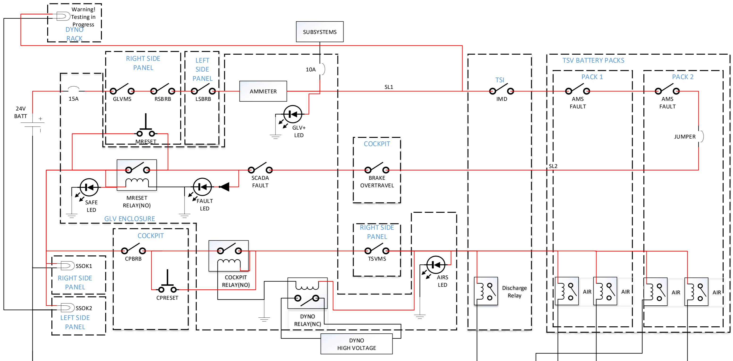
Safety Loop Diagram v.8 Last Updated 04/17/2019
