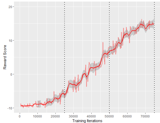
FIGURE 4. RL AGENT REWARD vs. TRAINING
